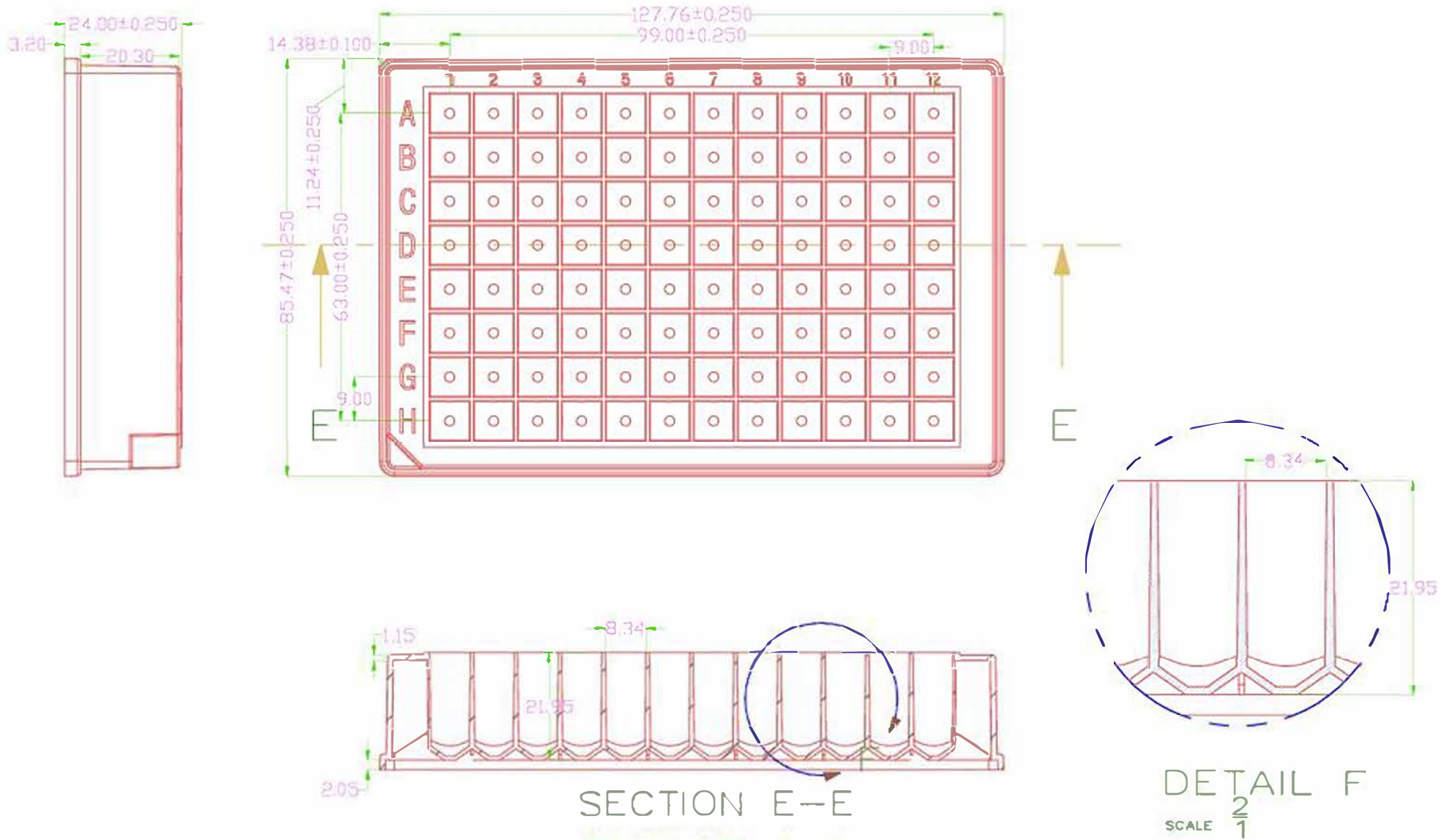
WB 2-4320 SafeStore 96 1.2mL Deep-well plate, Square wells, U-shape
